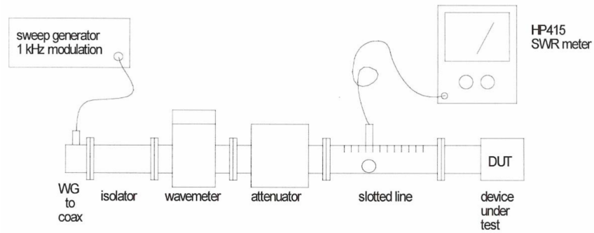
Figure 12.9: An experimental setup for a slotted line measurement (courtesy of Pozar and Knapp, U. Mass [82]).
